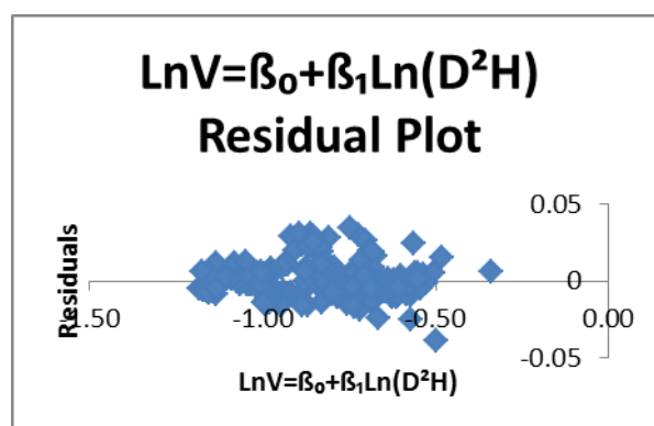
Figure 1: Residual Plot for the Observed versus Predicted for the Logarithmic Single Combined entry
