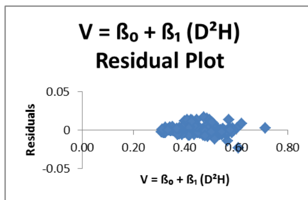
Figure 2: Residual Plot for the Observed versus Predicted for the Single Combined entry
